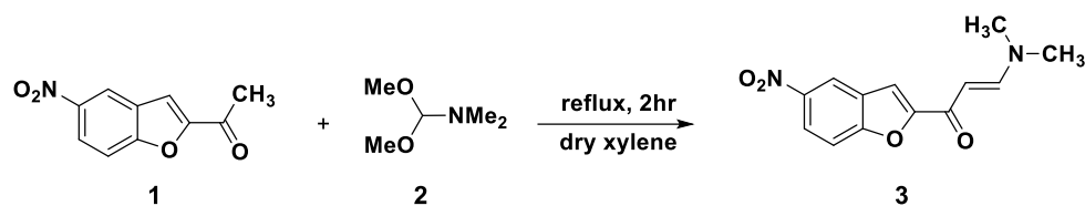
Scheme 1. General synthetic route from ketone 1 to enaminone 3 and the derived heterocycles.
