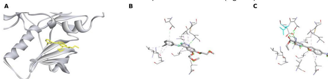
Figure 4. Three-dimensional binding modes of (A) crystallographic AQ4, (B) compound 10, and (C) compound 11 within the EGFR tyrosine kinase binding pocket. The panels illustrate the relative accommodation of the ligands inside the validated binding region. Green dashed lines indicate predicted hydrogen-bonding interactions where displayed.
